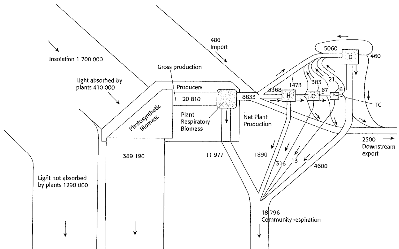
Fig. 3.39 The energy flow values in Silver Springs community. Units \text{kcal m}^{-2} \text{yr}^{-1} (1 kcal = 4.2 J)
